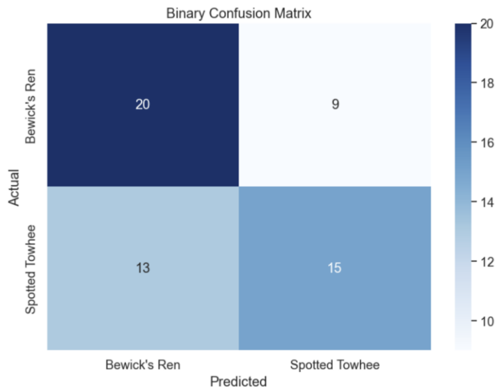
Figure 1 Binary Confusion Matrix
